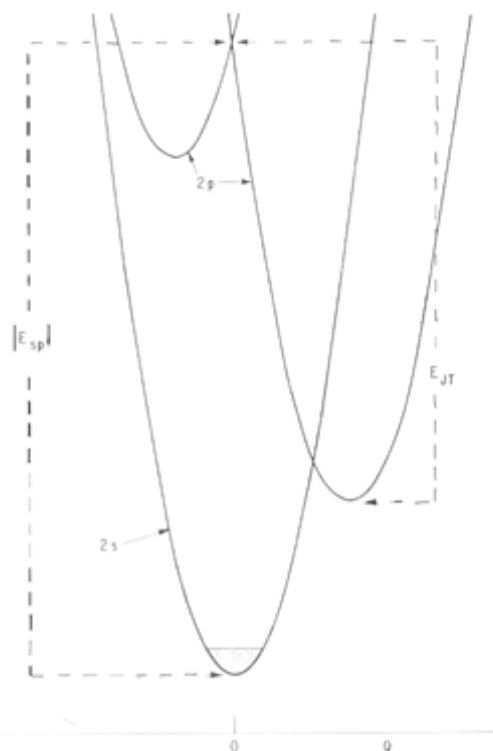
FIG. 1. Adiabatic energy surfaces for electronic 2s and 2p states as functions of a \Gamma_3^+ or \Gamma_5^+ distortion mode Q which splits the 2p degeneracy in first order (Jahn-Teller coupling). The figure illustrates the situation in which 2s is below 2p in the cubic configuration ( Q=0 ) by an energy difference |E_{sp}| and the Jahn-Teller energy E_{JT} of the 2p states is less than |E_{sp}| . The minima of the 2p energy surfaces in this case therefore lie above the minimum of the 2s surface, which occurs in the cubic configuration. There is no coupling of the 2s and 2p states via a \Gamma_3^+ or \Gamma_5^+ distortion mode. The energy of the lowest vibrational state on the 2s surface is indicated by a horizontal line within the 2s well, which also shows the approximate spatial extent in Q of the vibrational wave function of this state.
